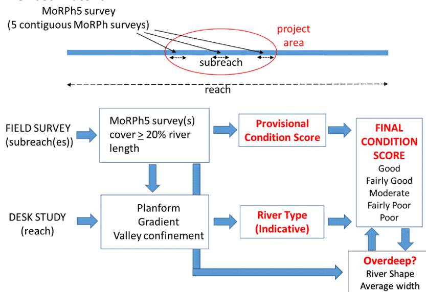
Figure 1 Reach and subreach scale components of the river Condition Assessment. Above: Schematic layout of reach and subreach scale elements. Below: Flow diagram illustrating how the Provisional Condition Score for a MoRPh5 subreach is translated into a Final Condition Score according to the (indicative) River Type.
